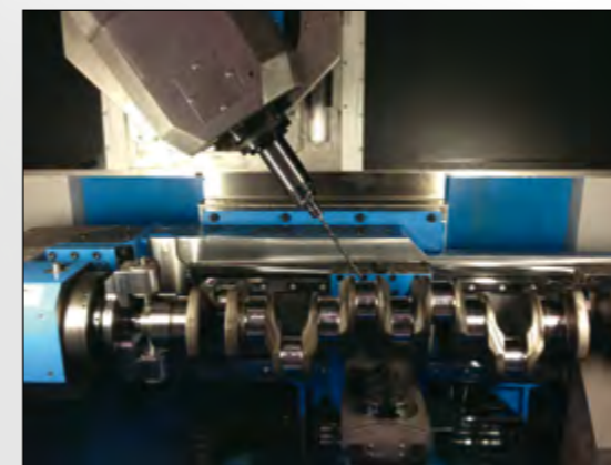
Infinitely tilting tool spindle and clamping device with turning module and C-axis, movable tailstock and movable support during the machining of longer crankshafts
